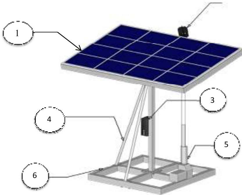
Gambar 3.1 : Single axis
