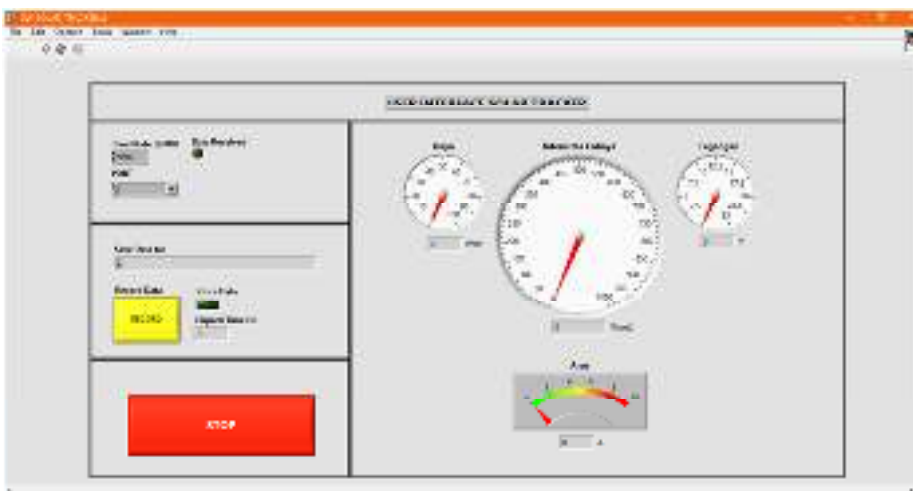
Gambar 3.16 : GUI_Solar_Tracker_V2.1.exe
